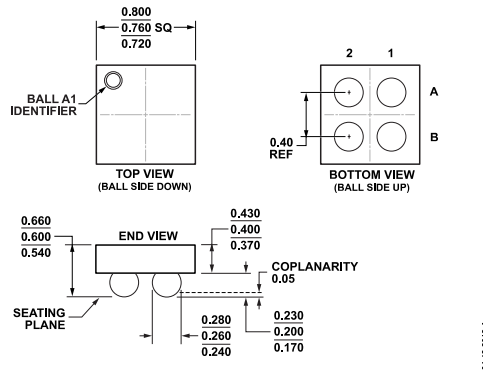
Figure 50. 4-Ball Wafer Level Chip Scale Package [WLCSP] (CB-4-3) Dimensions shown in millimeters
